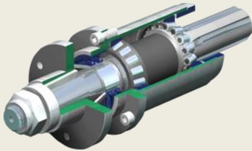
Tapered Roller Bearing
