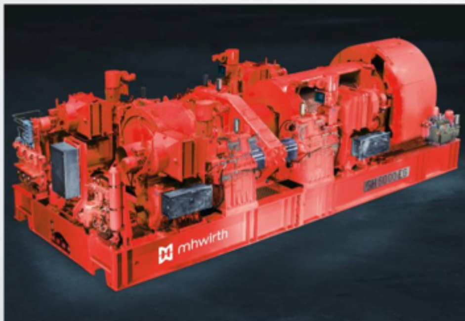
Drawworks 8000 hp
