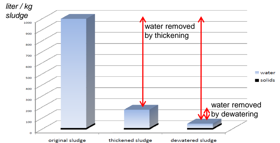
Sludge Dewatering with the HUBER Screw Press Q-PRESS®
