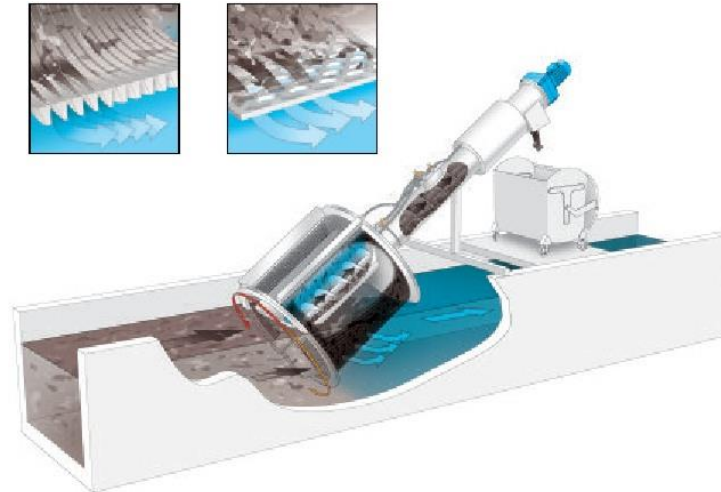
HUBER ROTAMAT® Drum Screens (Fine Screening Applications)
