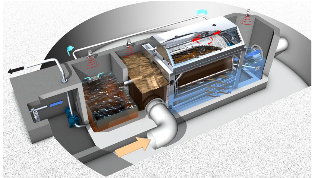
HUBER CarbonWin® Process for Primary Clarifier Replacement
